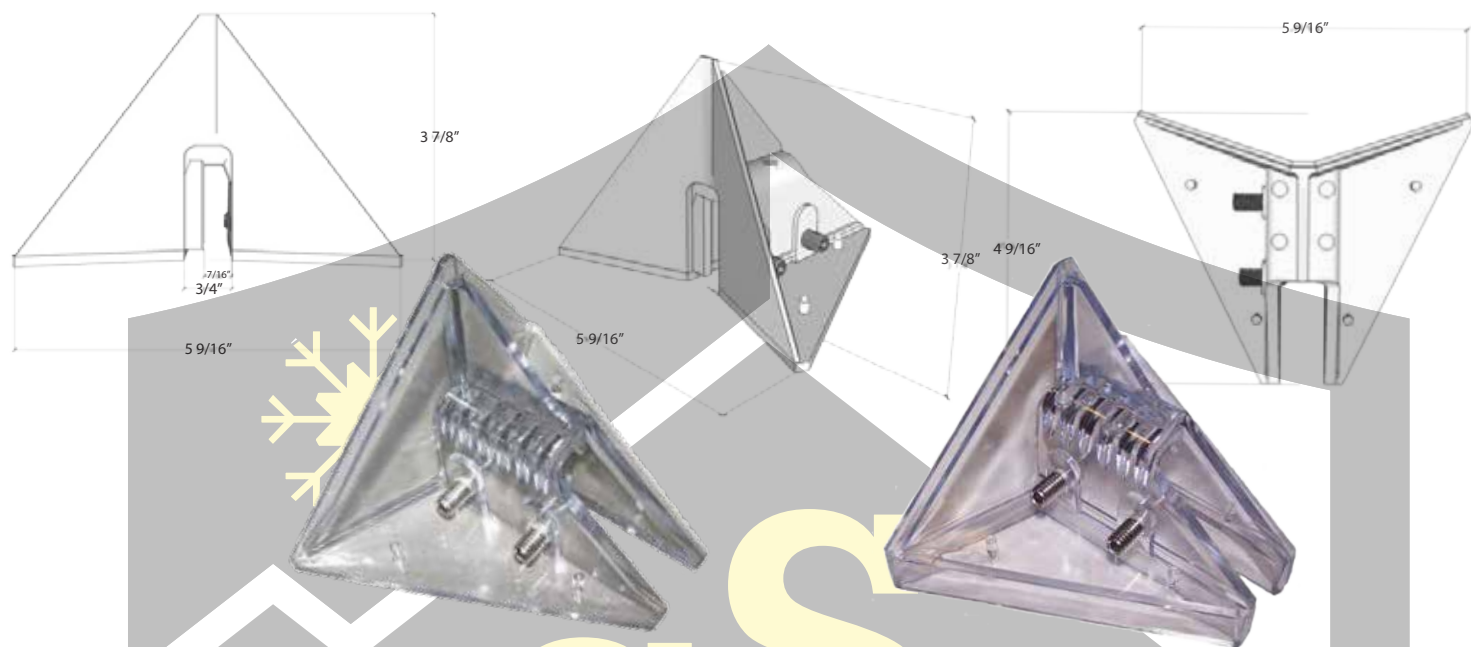
Rib Guard 1 Rib height up to 1 1/2"
